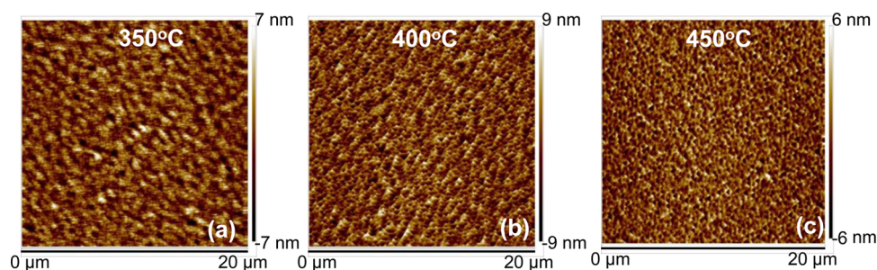
Figure 3. Surface morphology of the epitaxial Ge layers grown at three different growth temperatures on (100)/2° GaAs substrates. The measured surface roughness are in the range of 1.8–2.5 nm.
