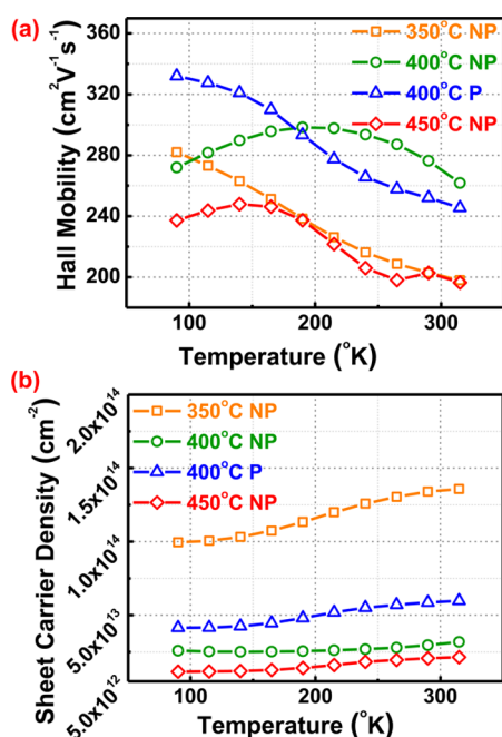
Figure 6. (a) Hall mobility and (b) sheet carrier density as a function of temperature in Ge layers grown at 350, 400, and 450 ^{\circ}\text{C} , respectively. Ge layers were grown with without pause (NP) and with a long growth pause (P).
